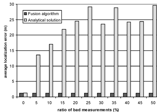
Fig. 15. The average localization error vs. the ratio of bad and good measurements.
