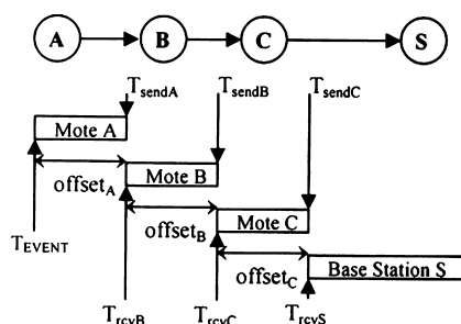
Fig. 7. Estimation of detection time T_{EVENT} can be iteratively determined along a routing path A, B, C, S as T_{rcvS} - \text{offset}_C - \text{offset}_B - \text{offset}_A . The horizontal axis is the timeline.
