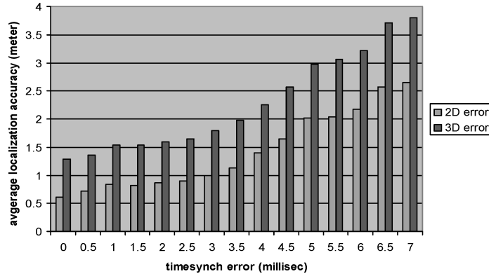
Fig. 10. Localization accuracy vs. time synchron error.
